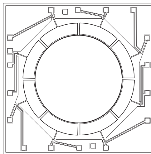
Figure 11.1 Silicon MEMS Ring
