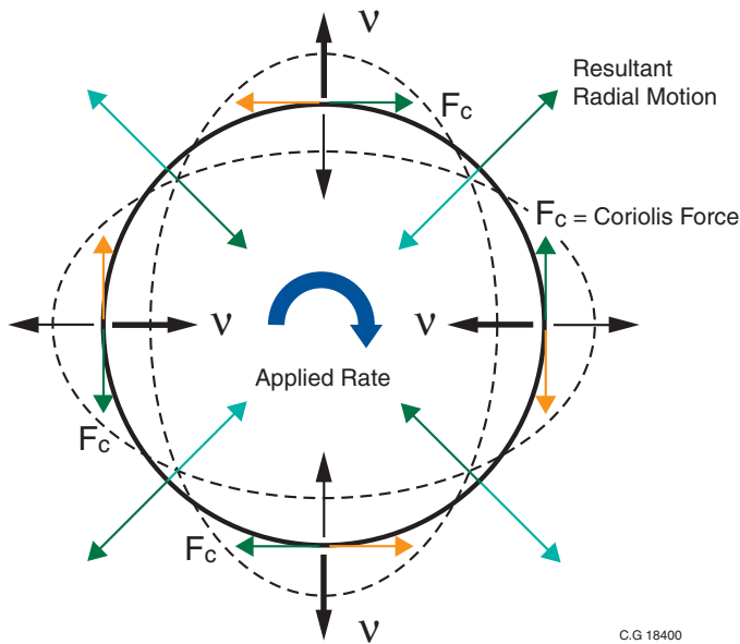
Figure 11.4 Secondary Vibration Mode
