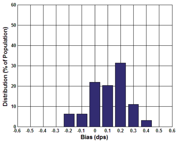
Figure 7.9 CRS39-03 Bias Setting Distribution (dps) at 45°C
